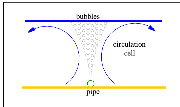
Figure 10: Sketch of air bubble curtain
